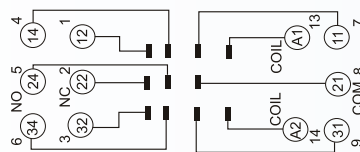
RELAY SOCKET SRN-11-SOK
