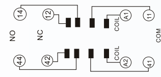
RELAY SOCKET SRN-14-SOK
