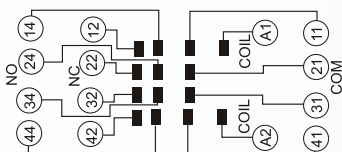
RELAY SOCKET SRN-08-SOK
